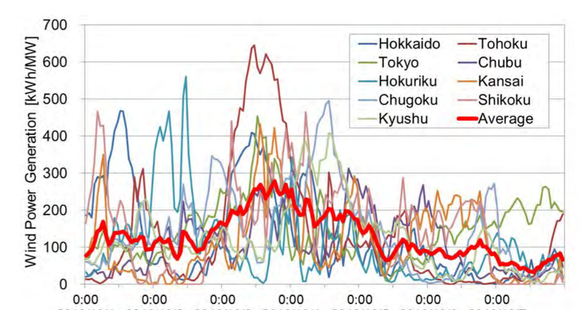
Variation of Wind Power Generation
