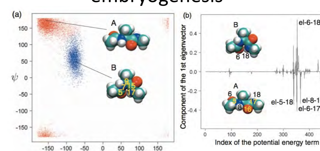
Fig. 3 Potential energy PCA analysis of peptide folding
