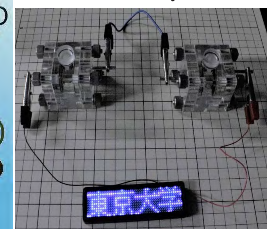
Prototype of the metal-air battery
