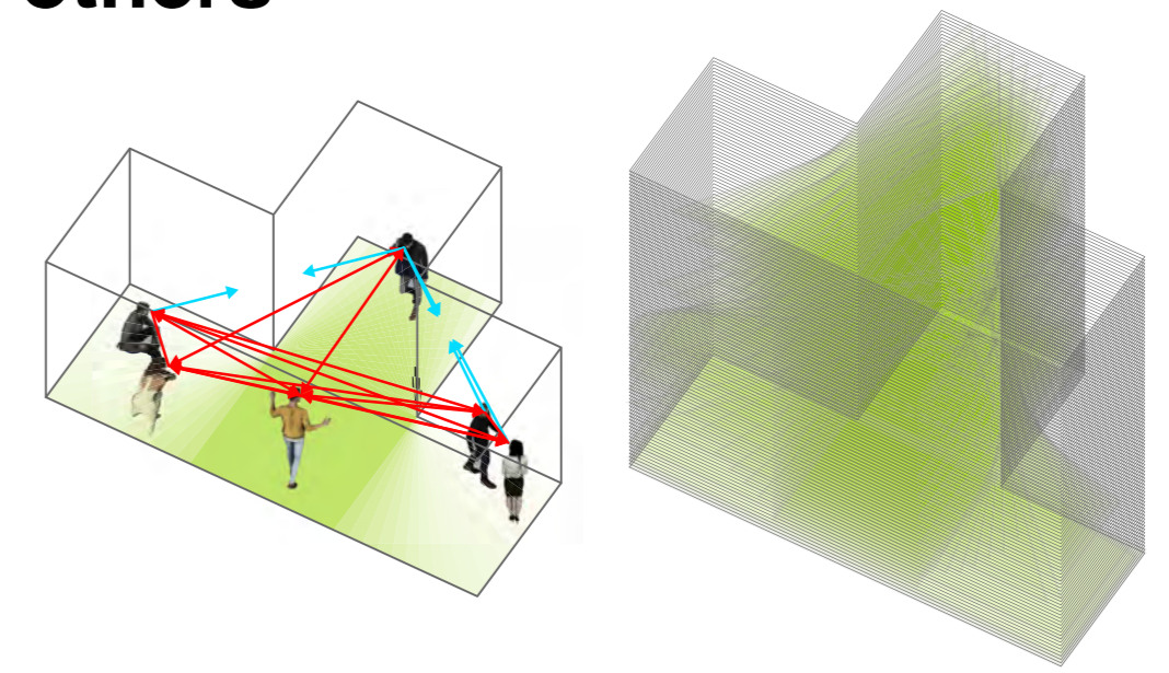
Convexhulls
