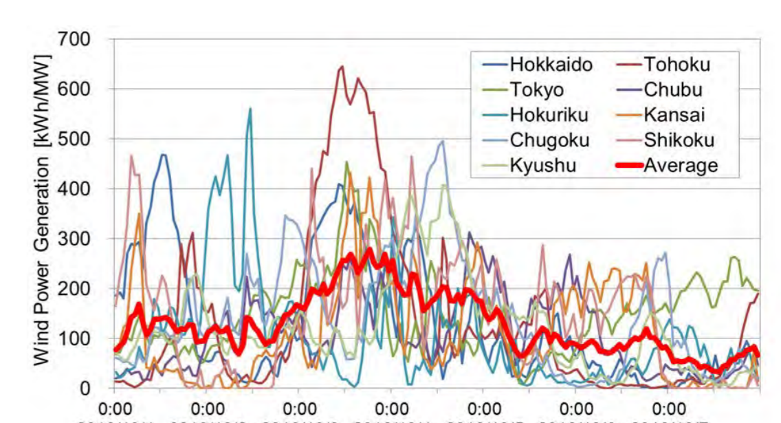
Variation of Wind Power Generation
