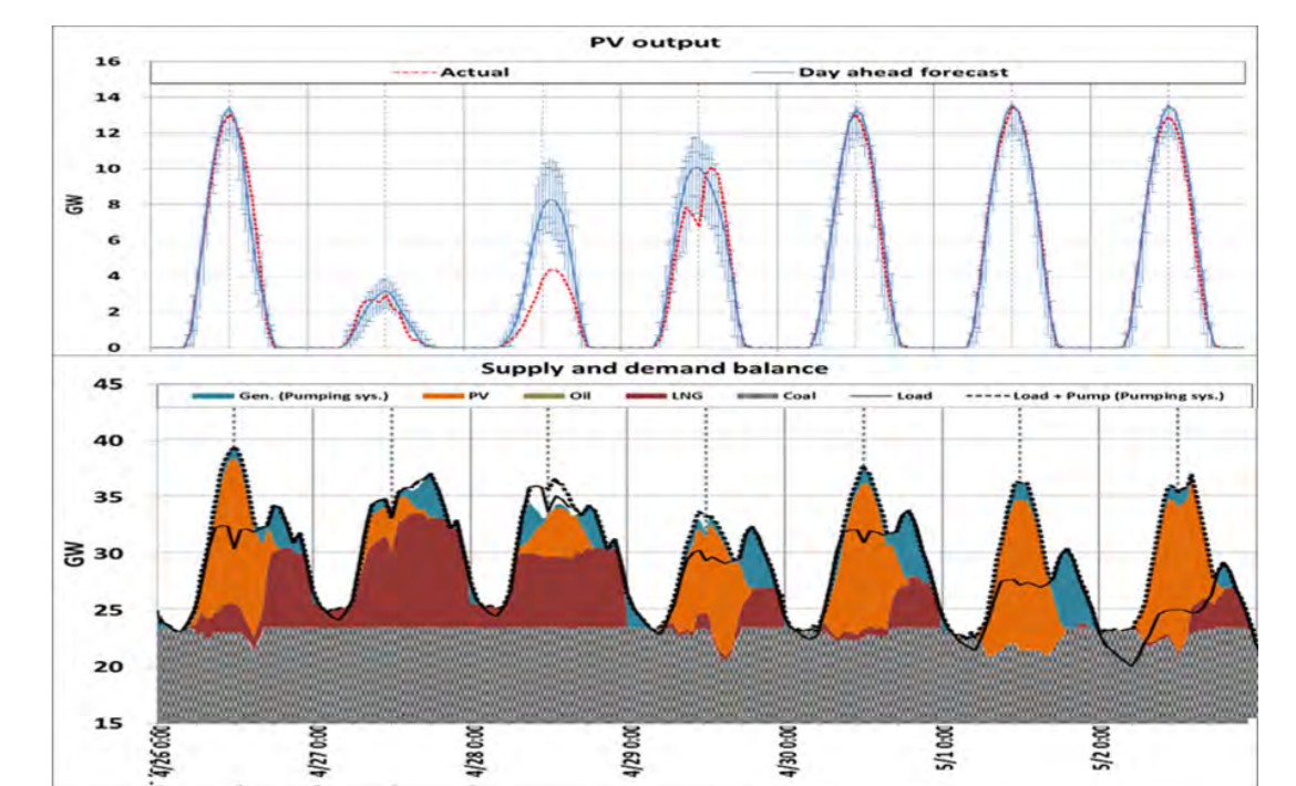
PV generation forecast, UC and Economic Load Dispatch
