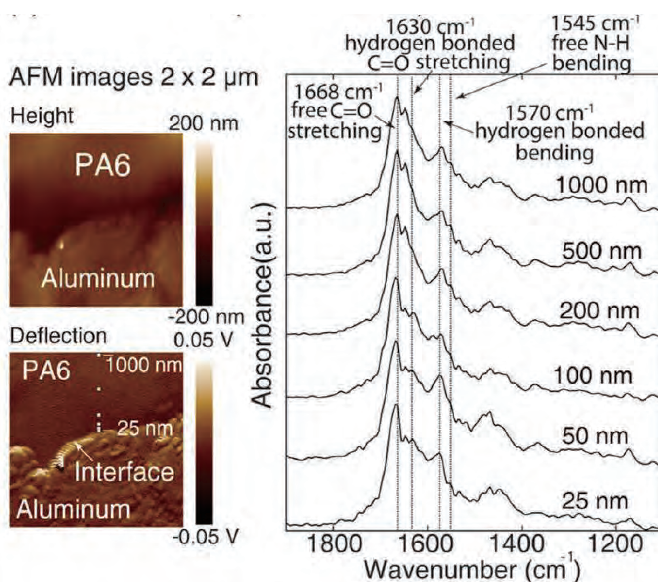
Hydrogen Bonding Spectra at the Interface of Al/PA6 Molding Joint
