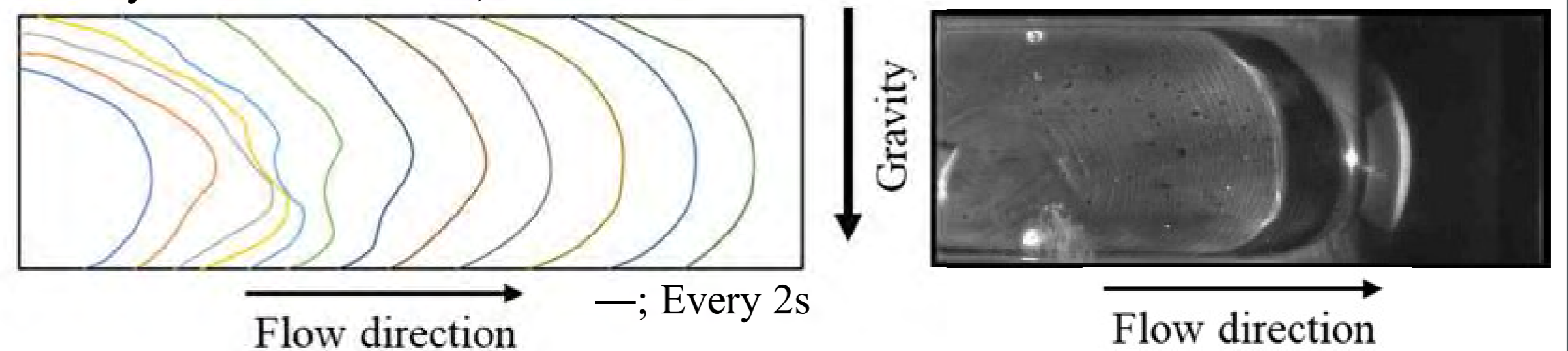
Filling pattern observed through parting line side
