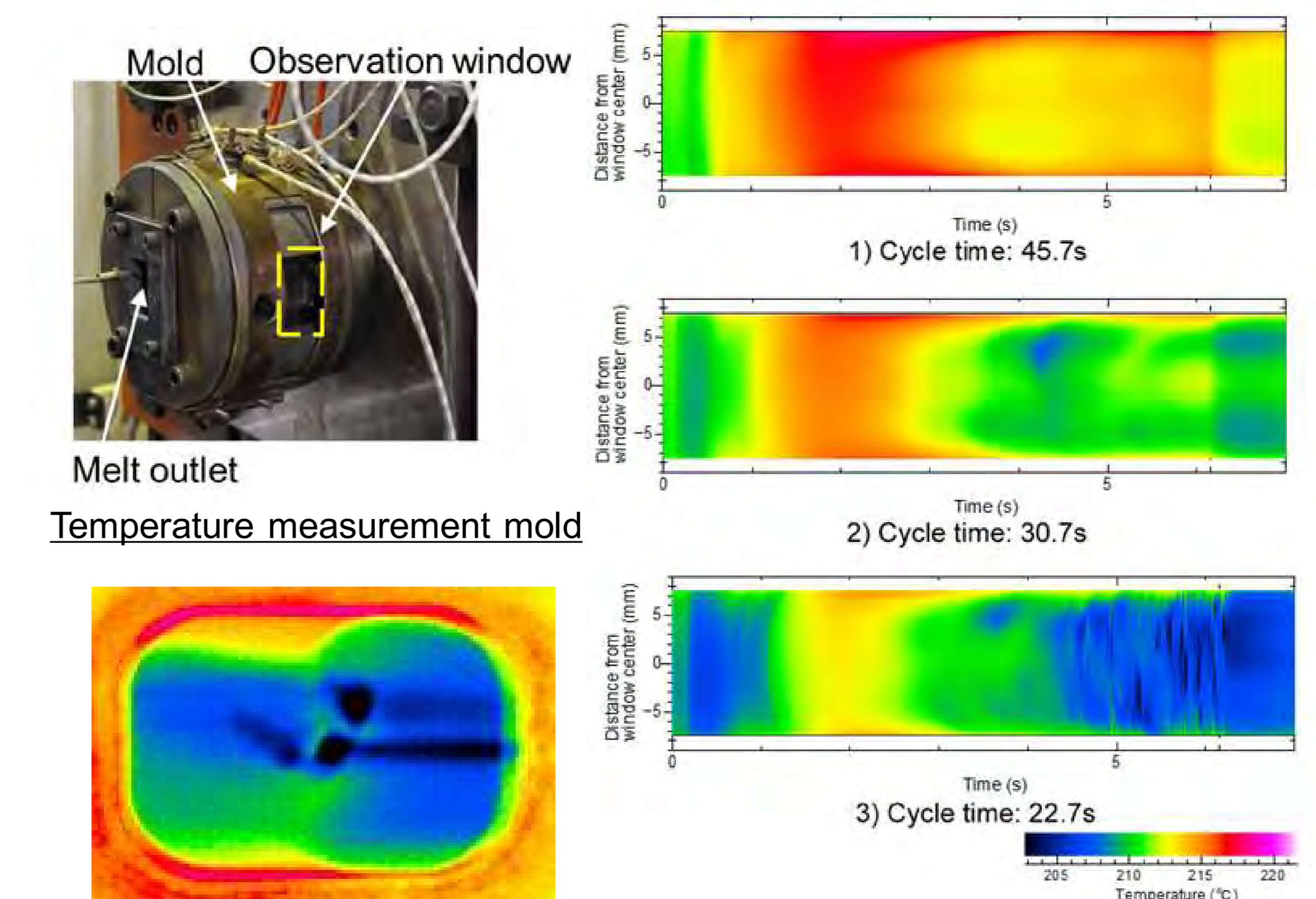
Thermal image of low temperature resin inflow (polypropylene)
